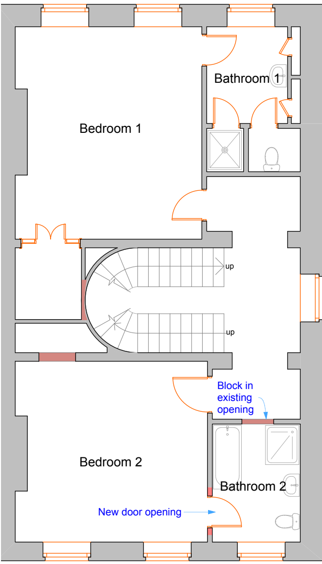
First Floor
