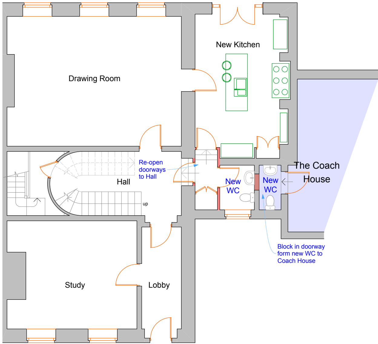
Ground Floor
