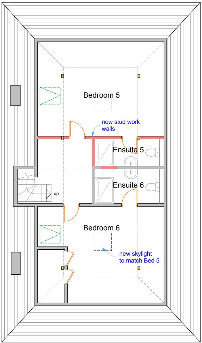
Third Floor
