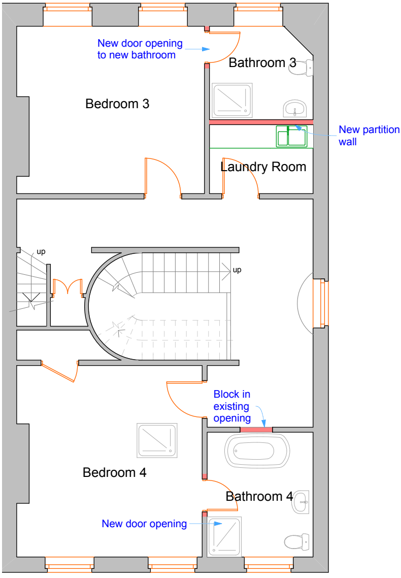
Second Floor
