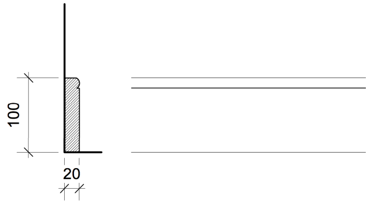
Section Elevation Routed, painted MDF Skirting: Basement and Second Floor
