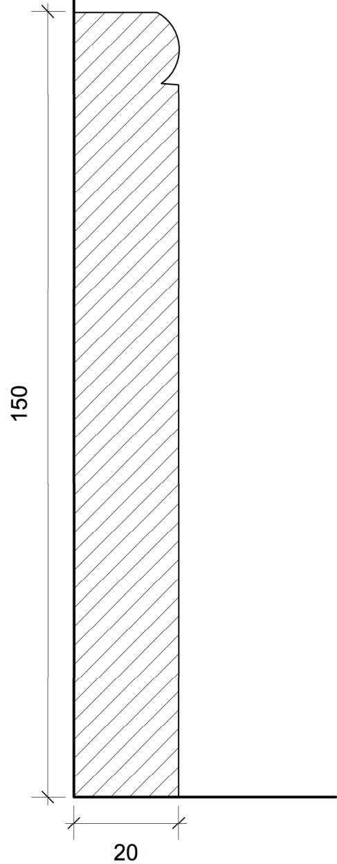
Skirting Detail 1:1 @ A3
