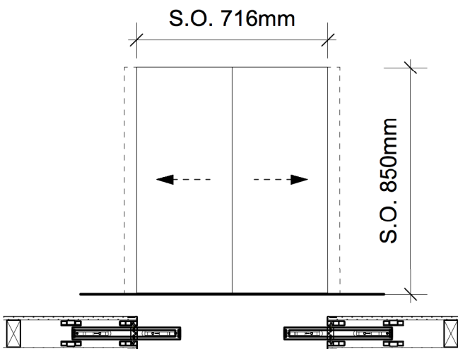
Door Type N D2.05 Second Floor - Family Bathroom Storage Painted, MDF-faced Pocket Door
