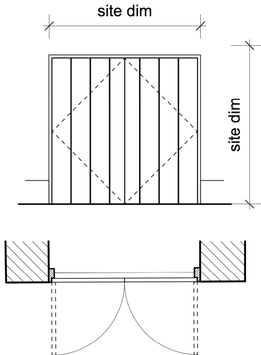
Door Type M D1.13 Second Floor - Master Bathroom Storage Painted, routed MDF-faced side-hung doors
