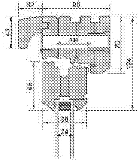
VENT & HEAD DRIP
