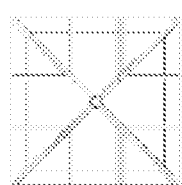
Standard Lantern - 6 Internal Upstand Size - 1660mm x 1660mm
