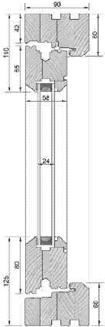
FLUSH CASEMENT
