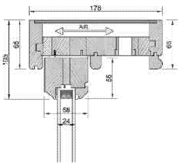
VENT & HEAD DRIP
