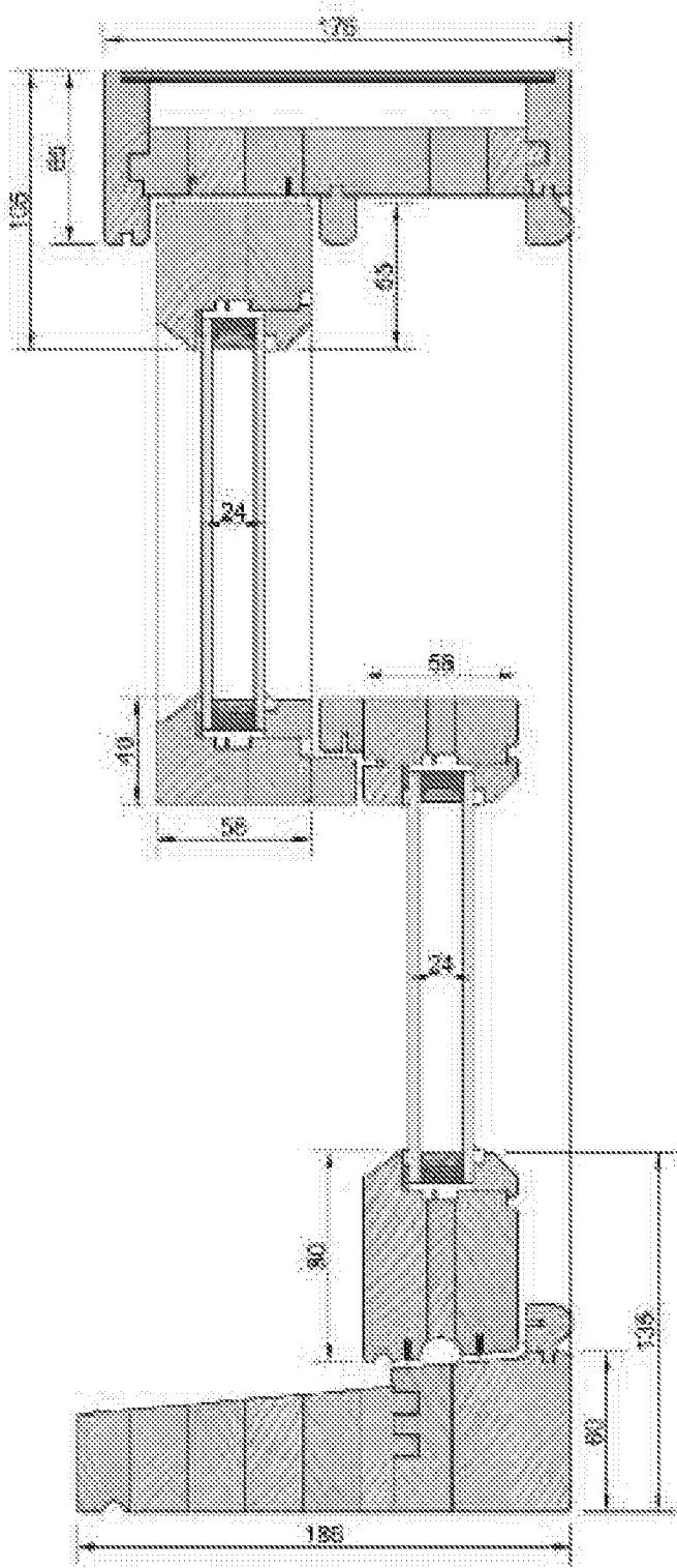
176 HIDDEN SPRING
