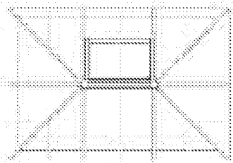
Standard Lantern - 1 Internal Upstand Size - 2295mm x 2205mm
