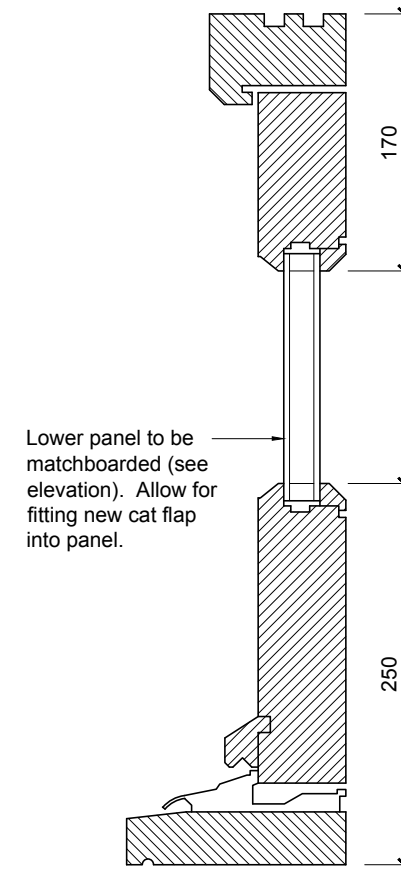
Vert Section thro New Back Door 1:5 @ A3
