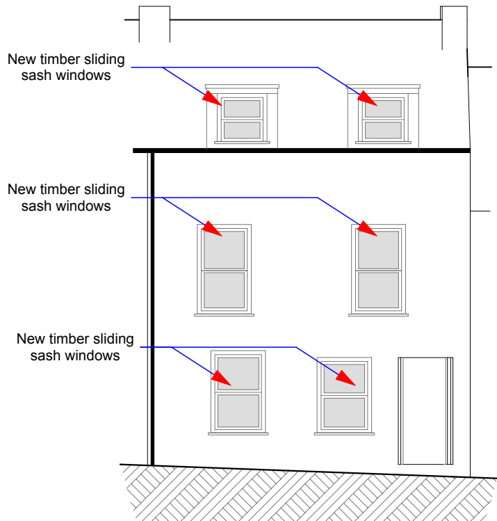
WEST ELEVATION
