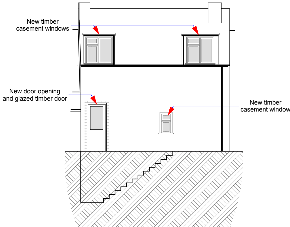
EAST ELEVATION
