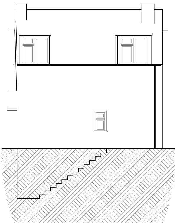
EAST ELEVATION
