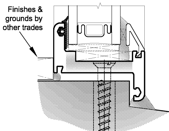
Direct Fix
