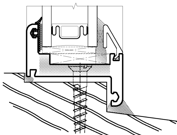
Timber Sub-frame
