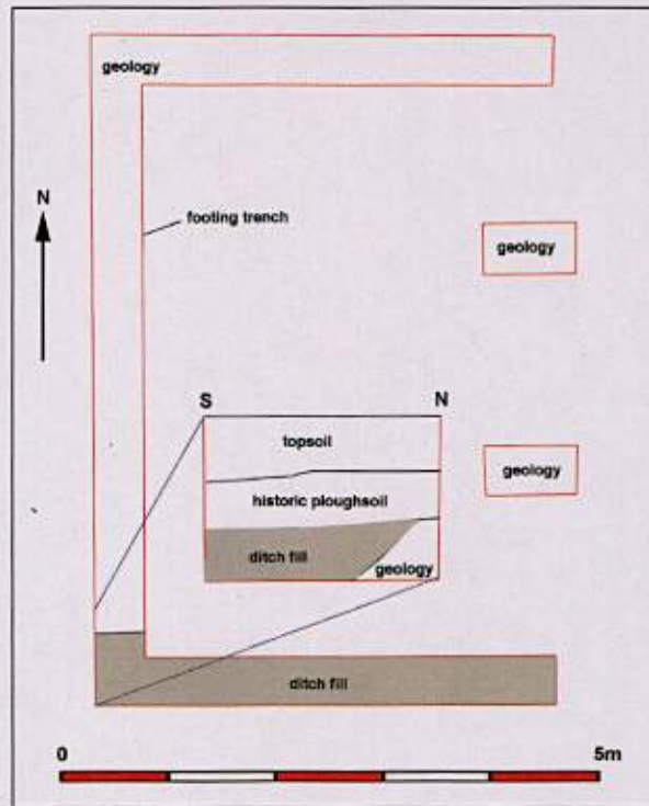
Figure 2 Plan of the excavated footing trench.
