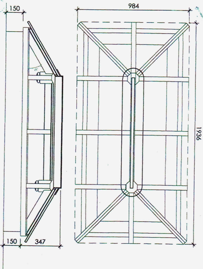
PROPOSED ROOF LIGHT SCALE 1:20
