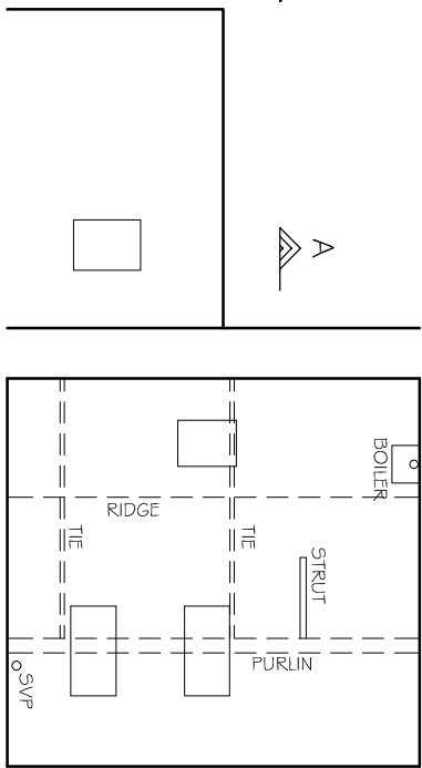
EXISTING ATTIC PLAN
