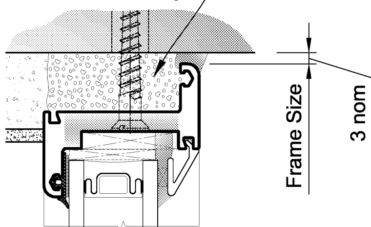
Direct Fix
