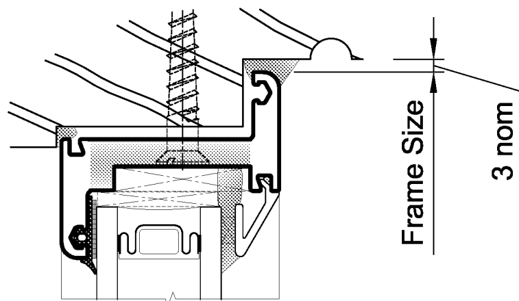
Timber Sub-frame
