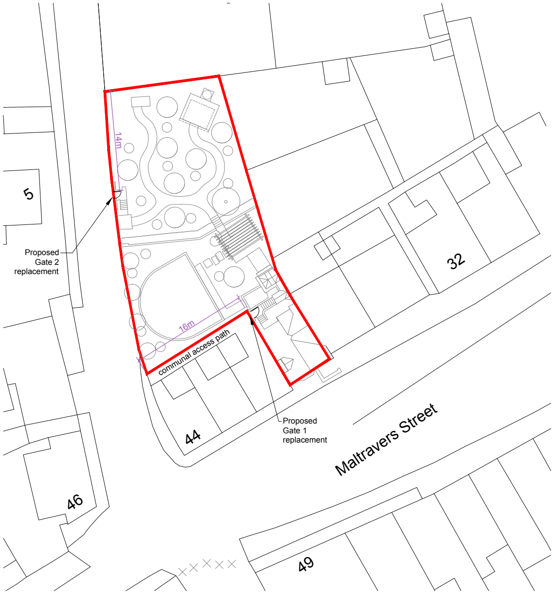
Block Plan 1:500
