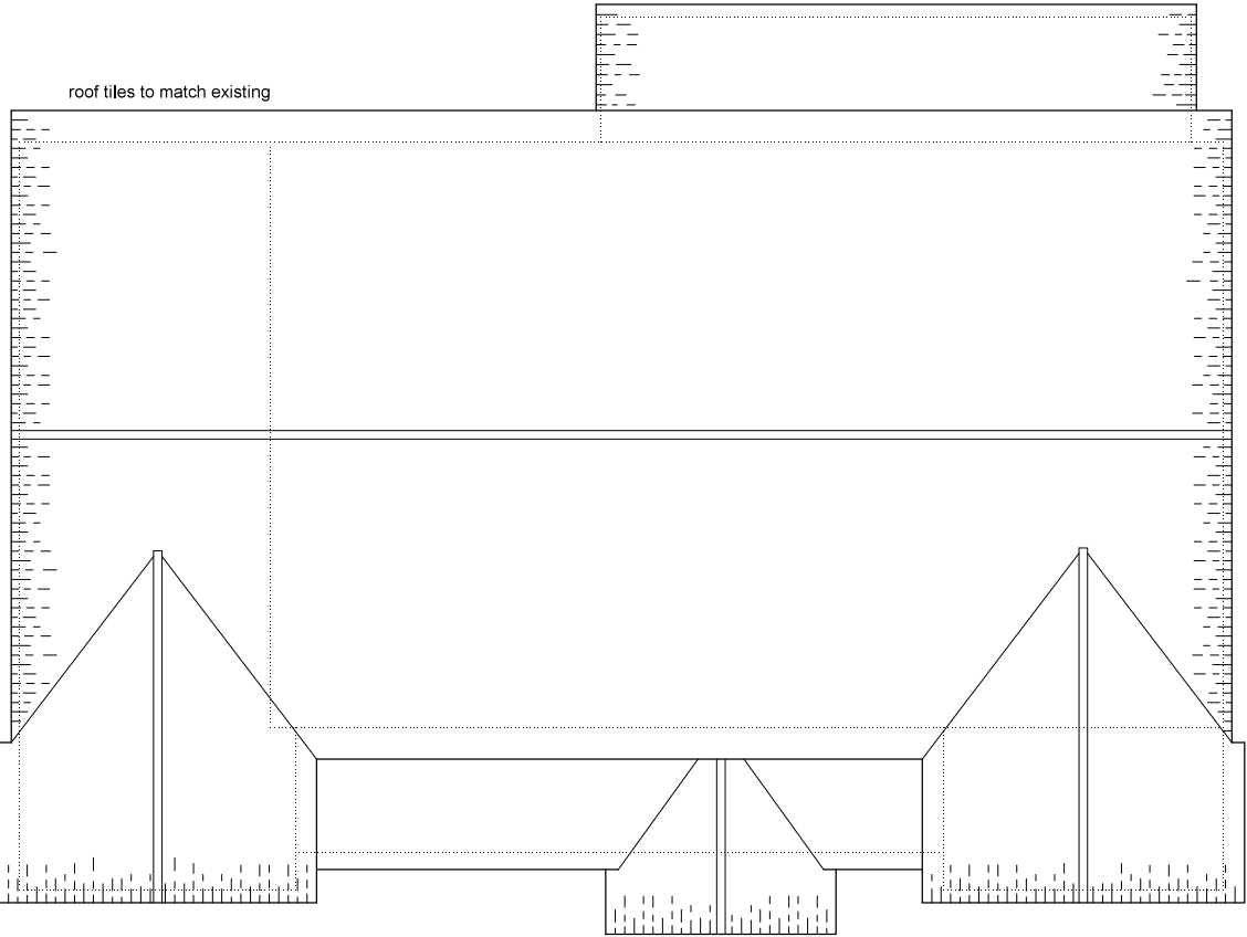
Roof Plan
