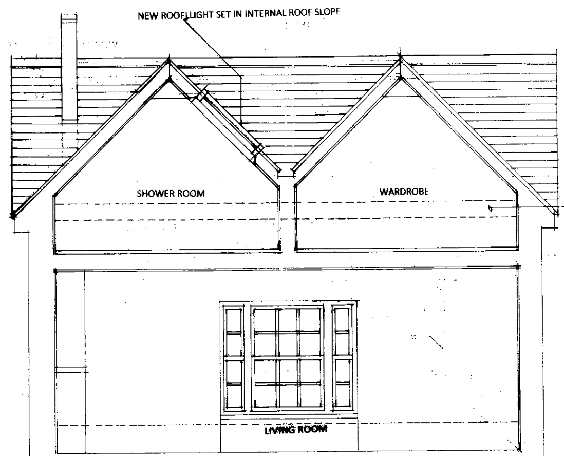
PROPOSED CROSS SECTION
