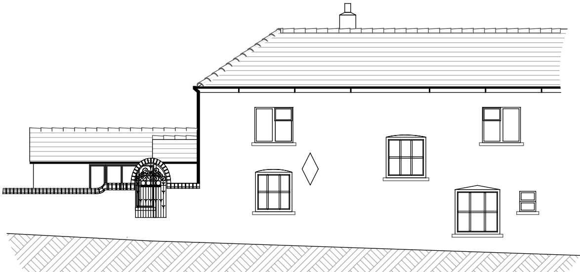
West Elevation
