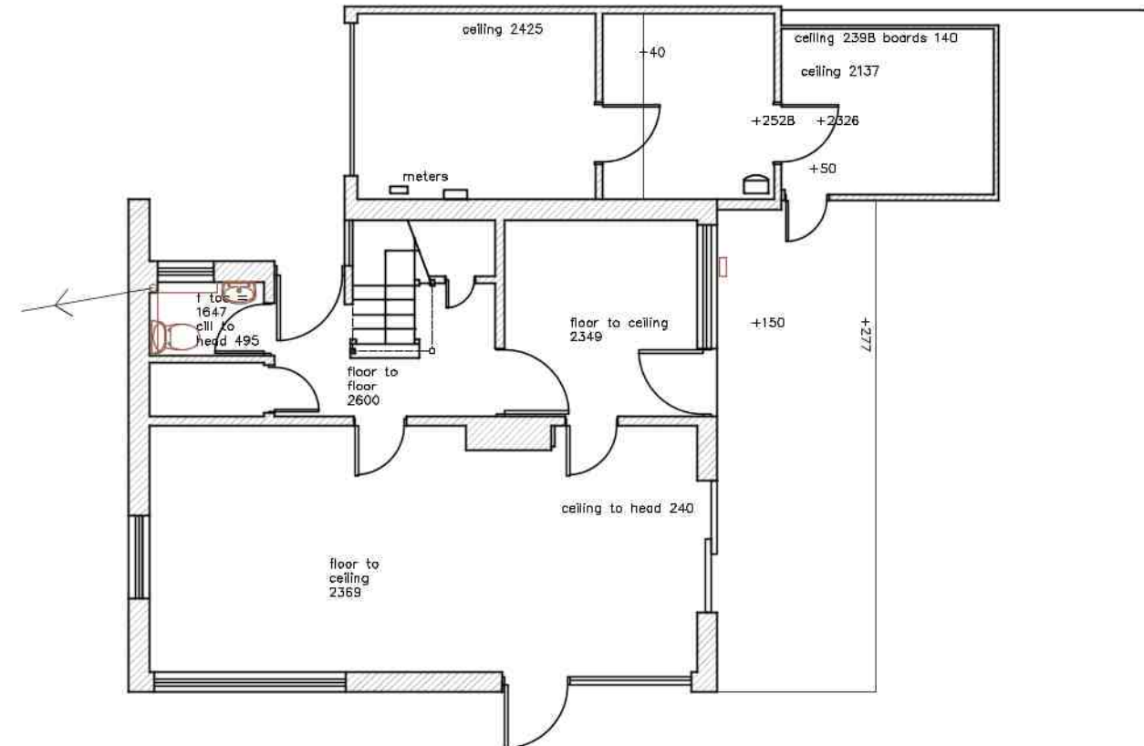
GROUND FLOOR PLAN [existing]
