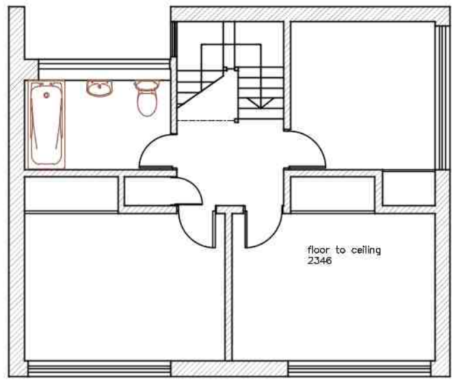
FIRST FLOOR PLAN [existing]
