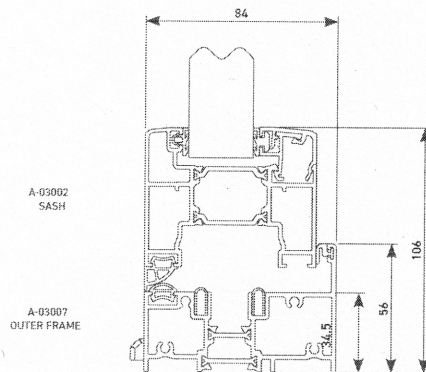
Standard outer frame with face drain
