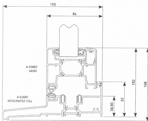
Integrated cill with sash profile
