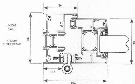
Outer frame and sash profile with hinge
