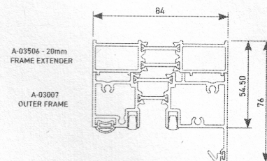
Standard outer frame with 20mm extender
