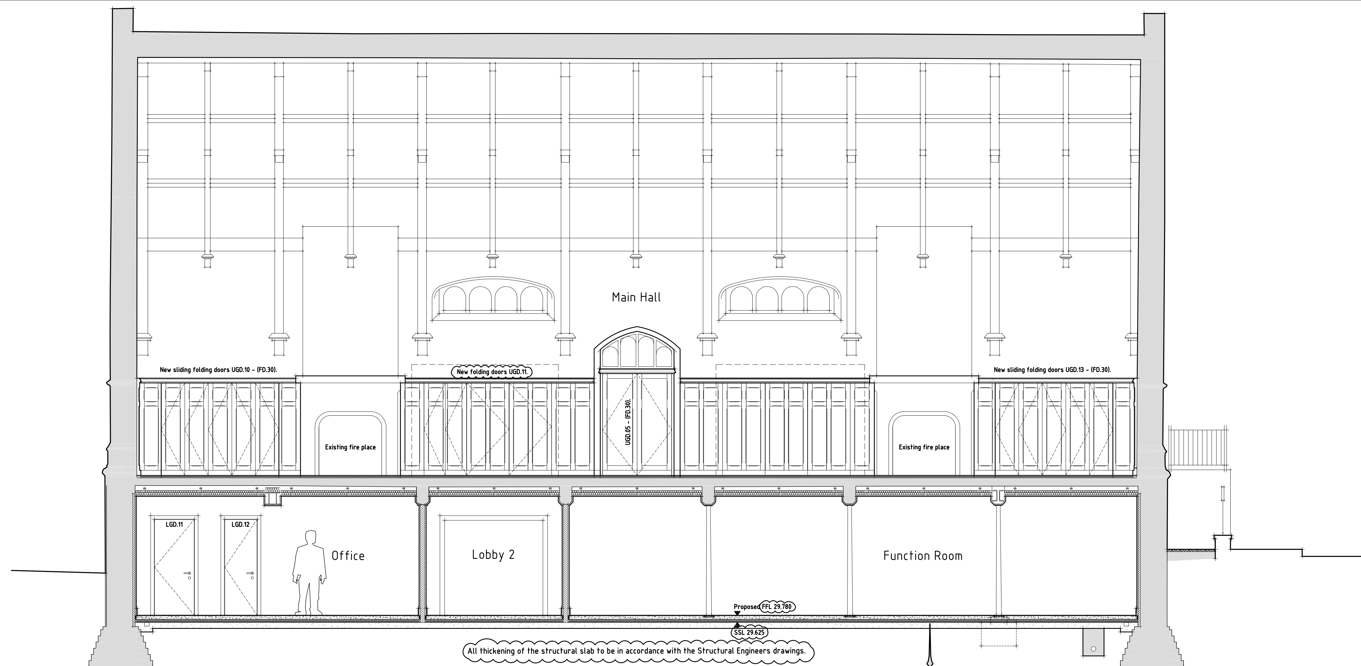
Proposed Section A-A
