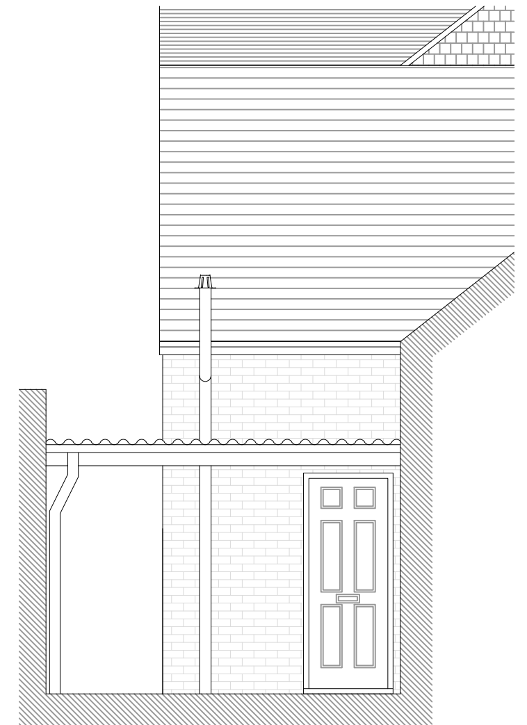
Section C-C EXISTING
