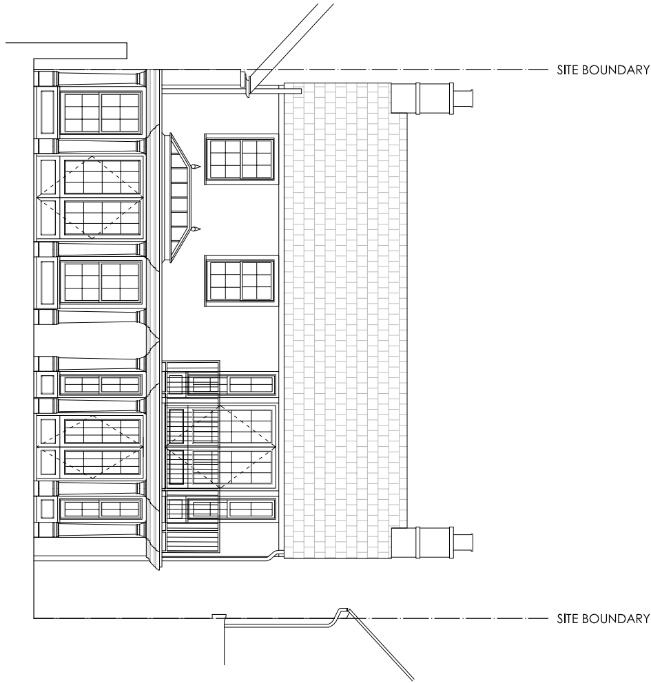
EXISTING SOUTH (REAR) ELEVATION SCALE 1:100
