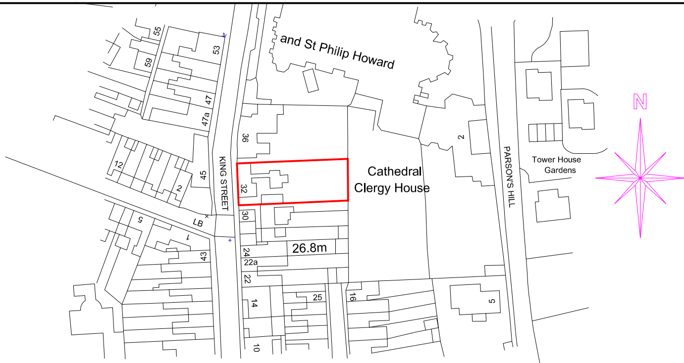
LOCATION PLAN - 1/1250
