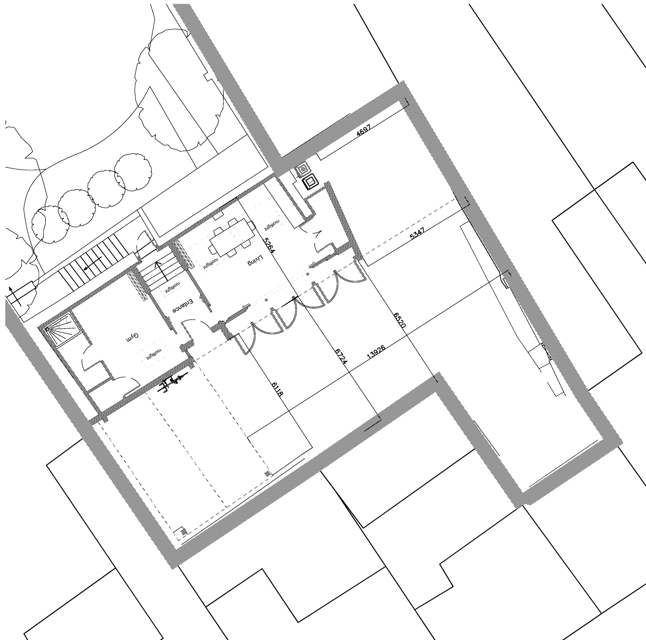
Dimensions to boundaries shown on proposed block plan 1:100 (@A2)
