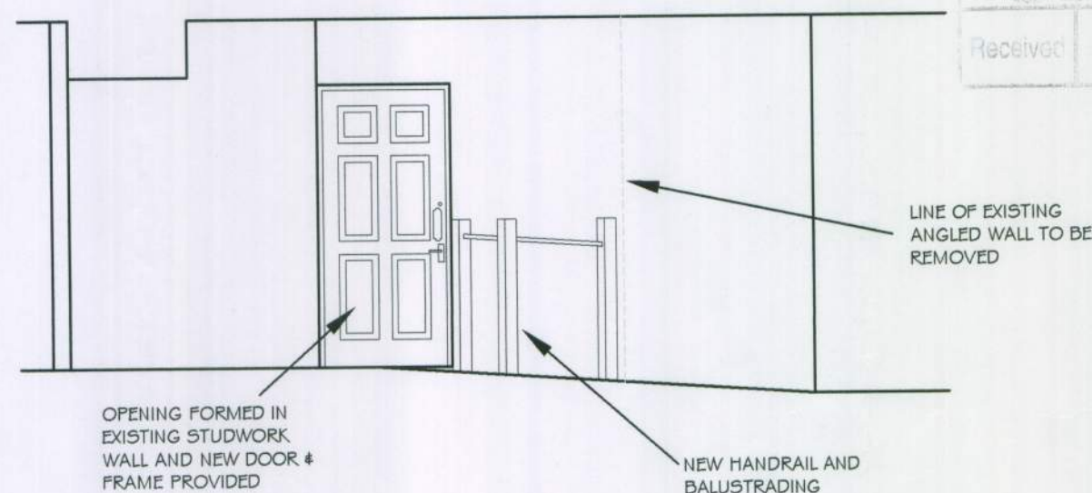
INTERNAL ELEVATION 1:50 (LOOKING FROM CORRIDOR TOWARDS NEW DOOR OPENING)
