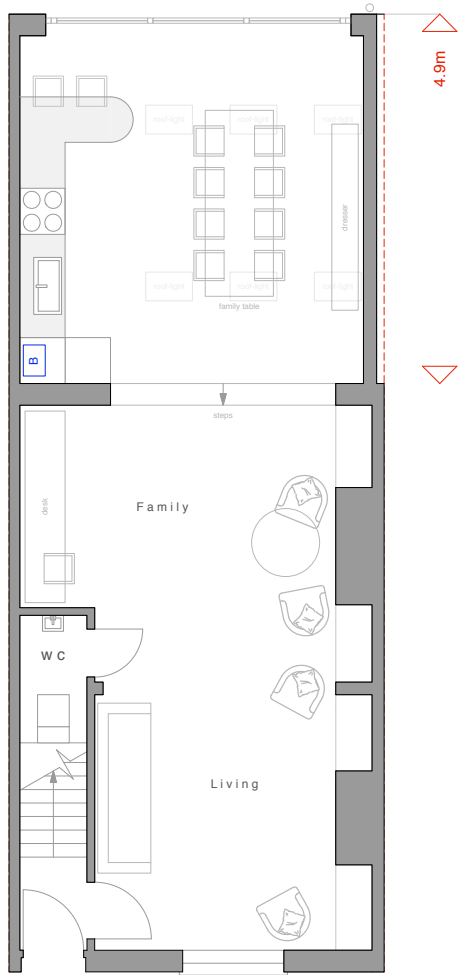
Proposed GF Plan at 1:100 scale
