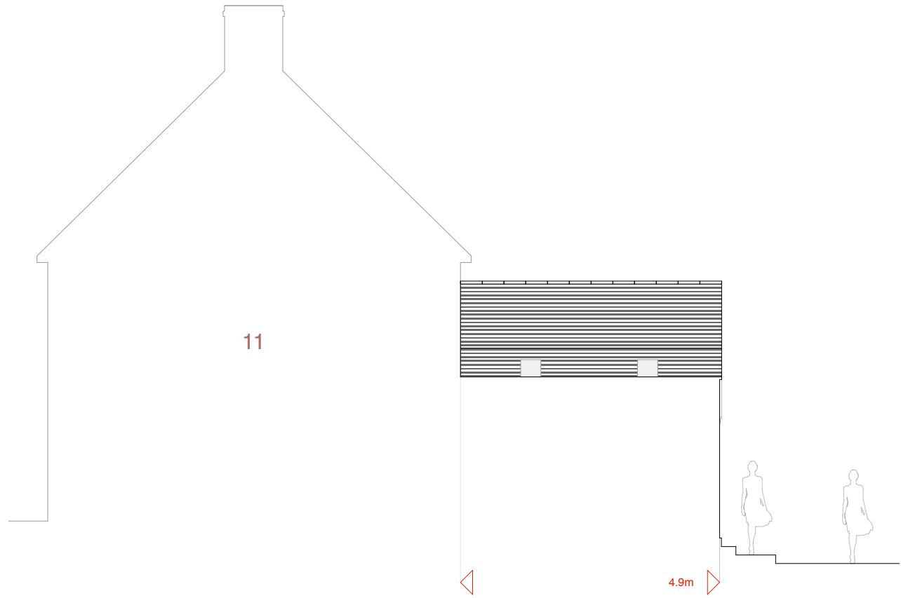
Proposed Side Elevation at 1:100 scale SOUTH WEST
