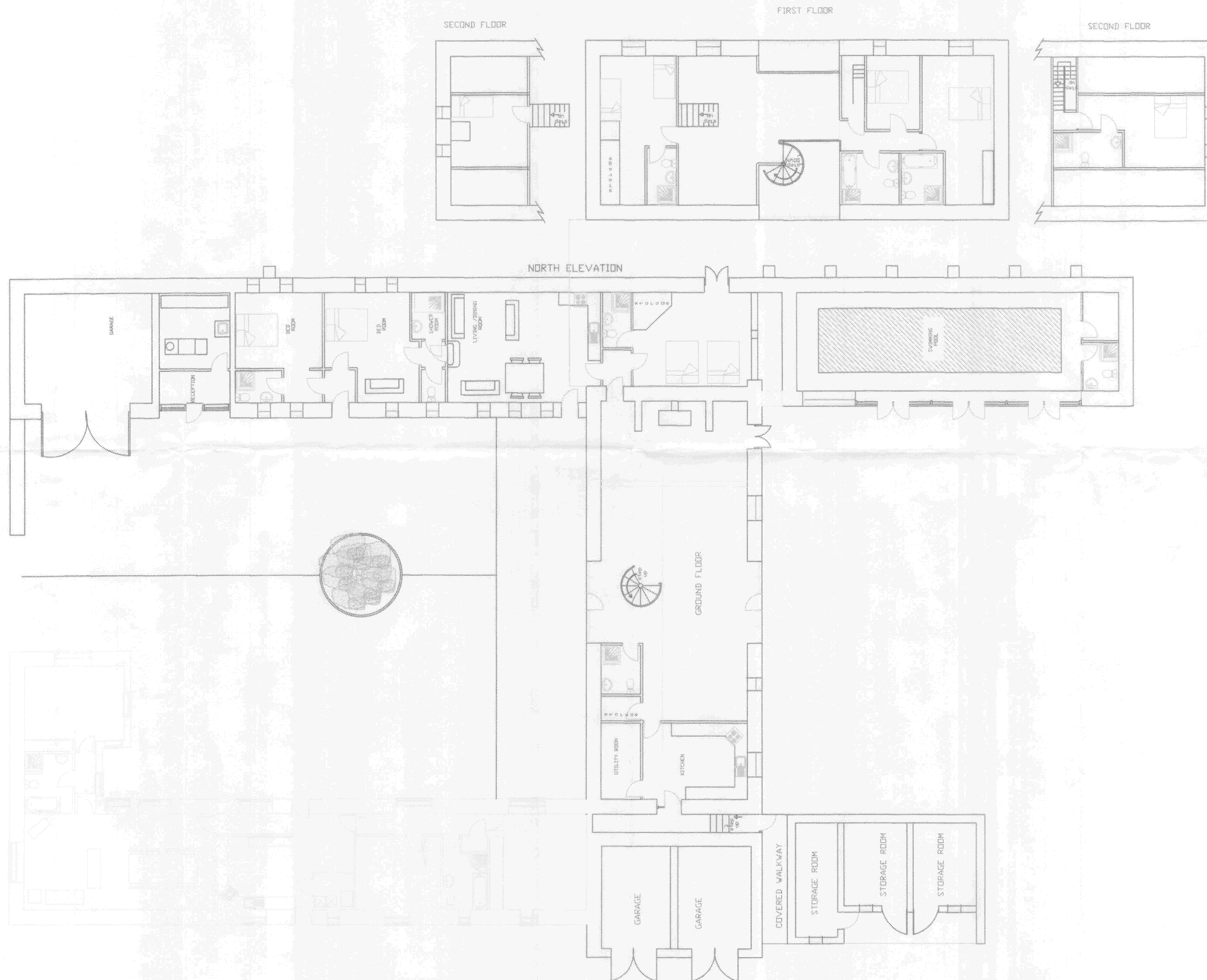
EXISTING FLOORPLANS 1:100
